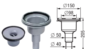
« The Vertical » made of ABS Vertical outlet Ø 50/40 1,2 l/sec flow rate* with odour trap for fitting in upper section sealing water height 50 mm 45 254
