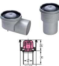
Practicus made of PP, with odour trap 1,8 l/sec flow rate*, sealing water height 50 mm Ø Lateral outlet Vertical outlet 50 45 150 45 250 75 45 170 45 270 110 45 110 45 210
